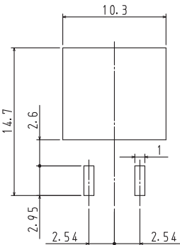
Land Pattern Example
