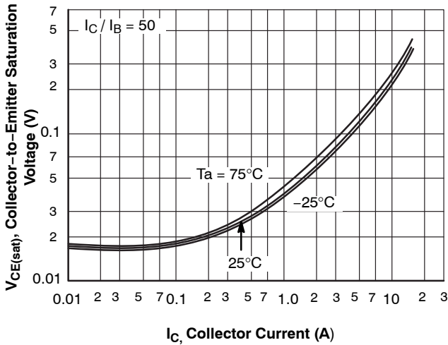
Figure 10. V_{CE(sat)} - I_C
