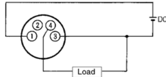
PNP Normally Open (F1-M3)
