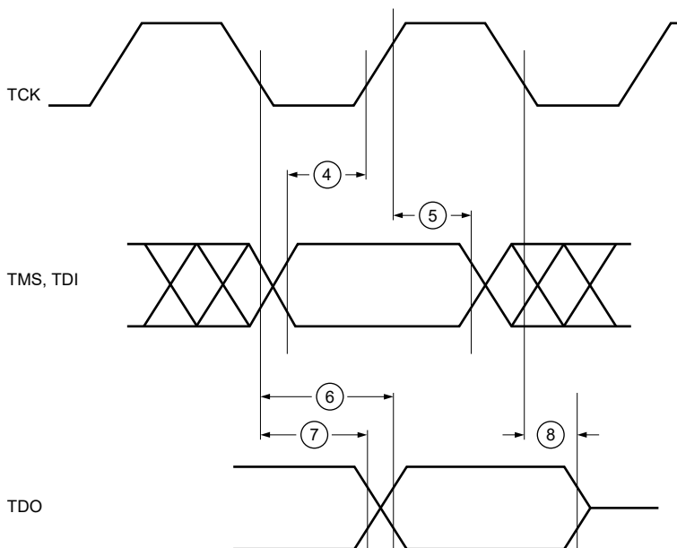
Figure 19. JTAG Test Access Port Timing
