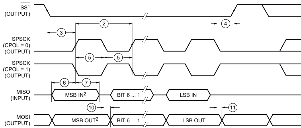
Figure 16. LPSPI Master Mode Timing (CPHA=0)
