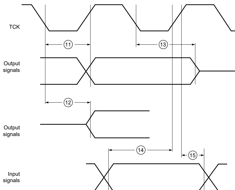
Figure 20. Boundary Scan Timing
