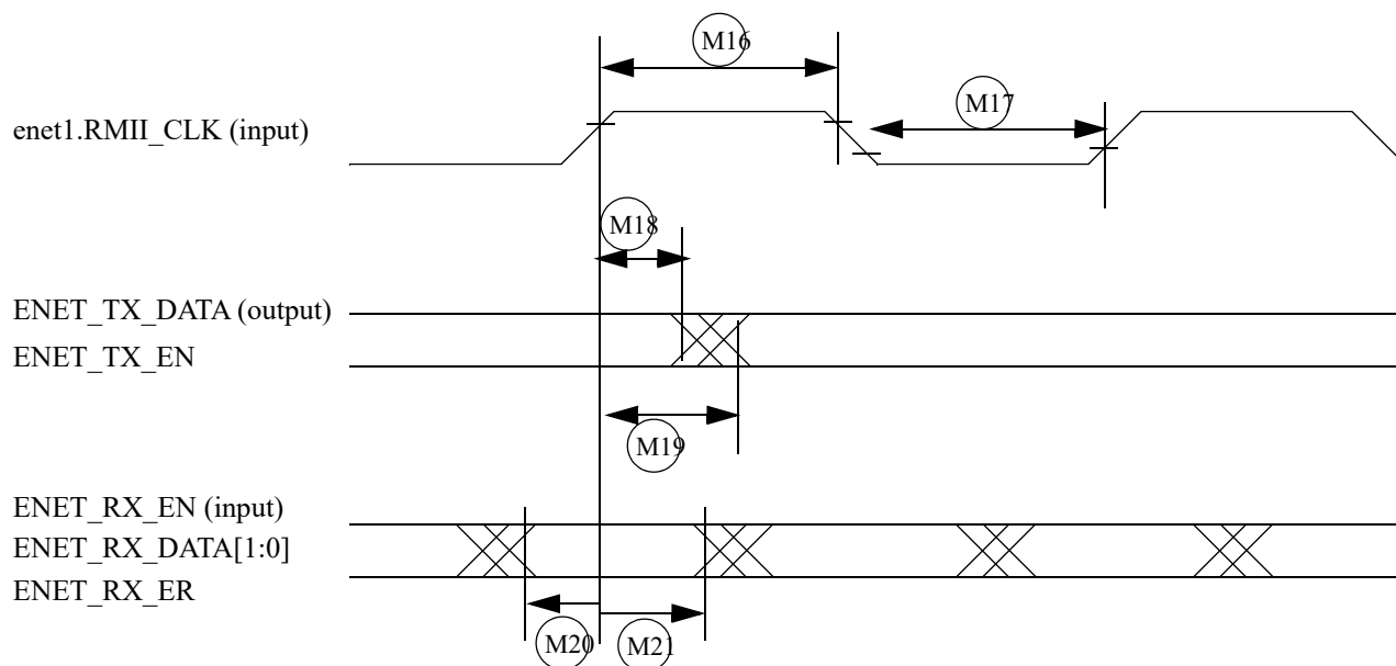
Figure 20. RII mode signal timing diagram
