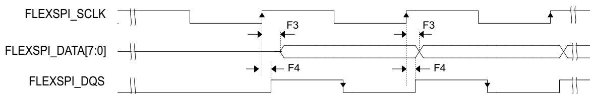
Figure 40. FlexSPI input timing in SDR mode where FlexSPI_MCR0[RXCLKSRC] = 0x3 (Case A1)
