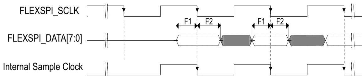
Figure 39. FlexSPI input timing in SDR mode where FlexSPI_MCR0[RXCLKSRC] = 0x0, 0x1, 0x2
