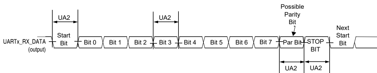
Figure 51. UART RS-232 Serial mode receive timing diagram
