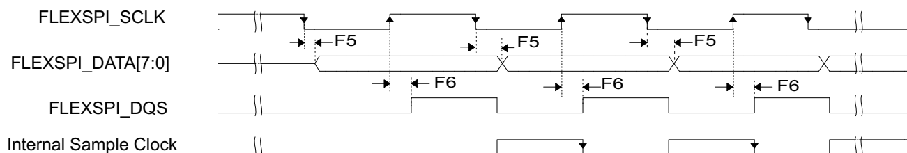
Figure 41. FlexSPI input timing in SDR mode where FlexSPI In _MCR0[RXCLKSRC] = 0x3 (Case A2)
