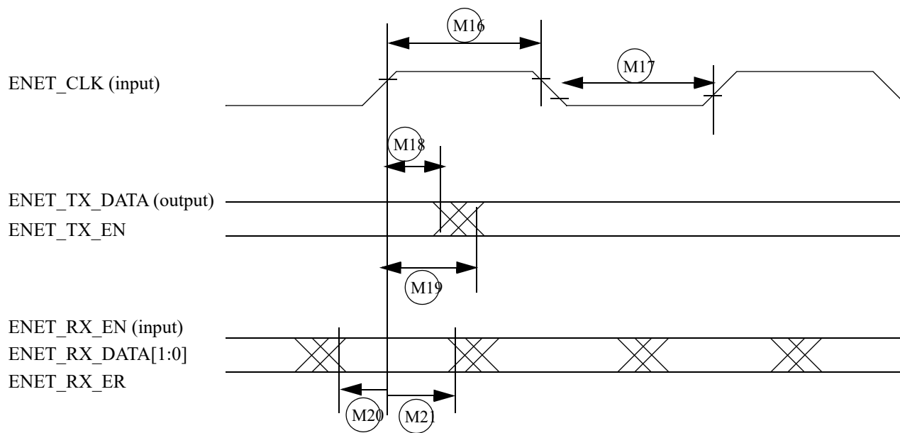
Figure 24. RMII mode signal timing diagram
