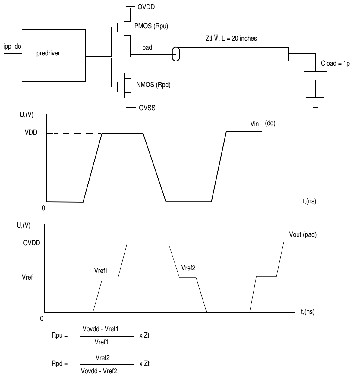
Figure 10. Impedance matching load for measurement
