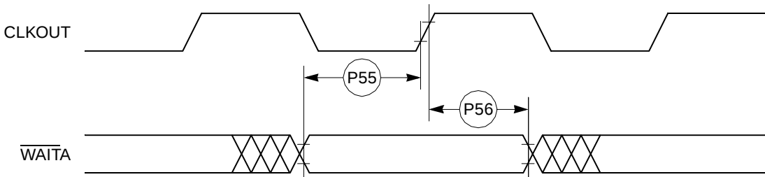
Figure 29. PCMCIA \overline{WAITA} Signals Detection Timing
