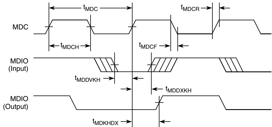
Figure 22. MII Management Interface Timing Diagram
