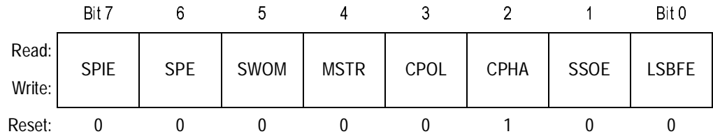
Figure 18-2. SPI Control Register 1 (SPICR1)
