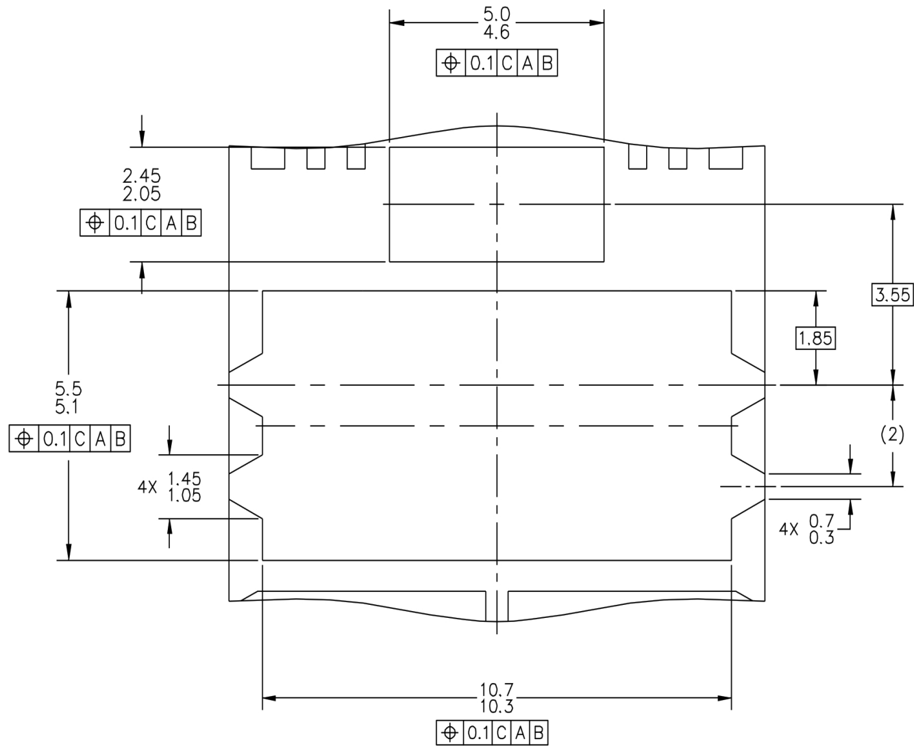
DETAIL F
