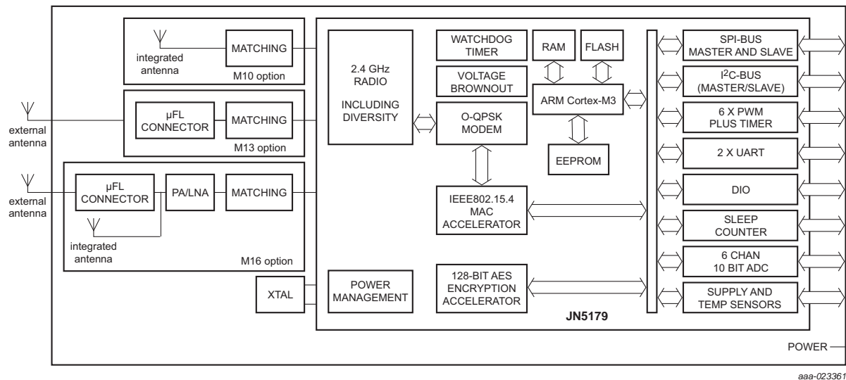
Fig 2. Block diagram
