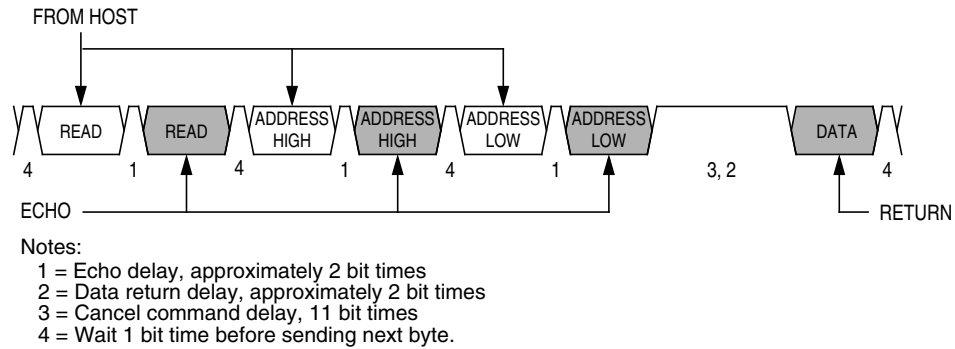
Figure 8-5. Read Transaction
