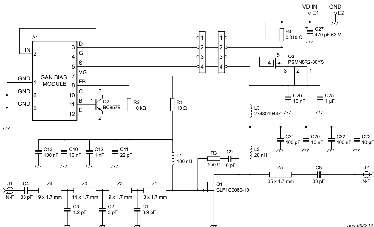
Fig 2. The broadband amplifier (500 MHz to 2500 MHz) demo circuit schematic
