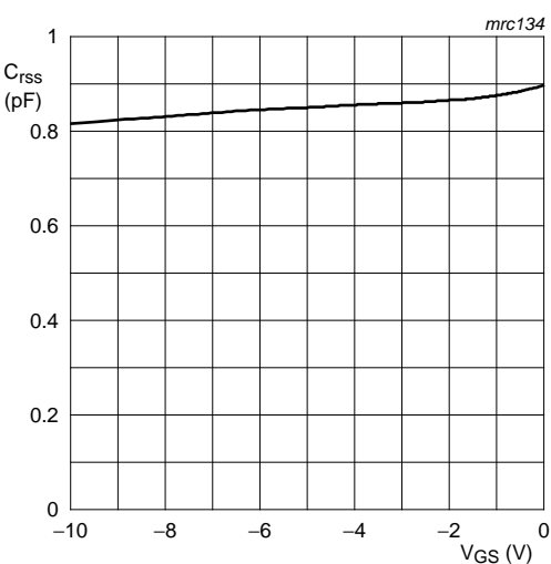
Fig 13. Reverse transfer capacitance; typical values.
