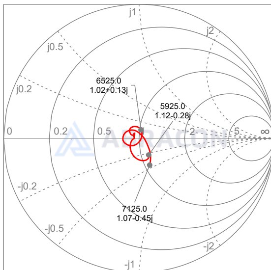
Smith chart S22 (5925~7125MHz)
