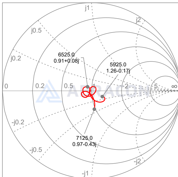
Smith chart S11 (5925~7125MHz)
