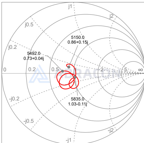
Smith chart S11 (5150~5835MHz)
