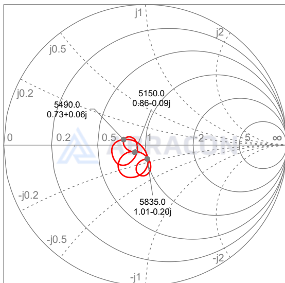
Smith chart S22 (5150~5835MHz)
