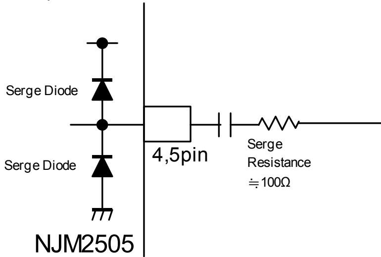
Fig1: External connection
