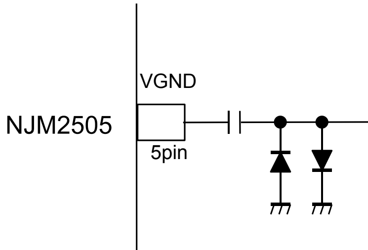
Fig4: External connection
