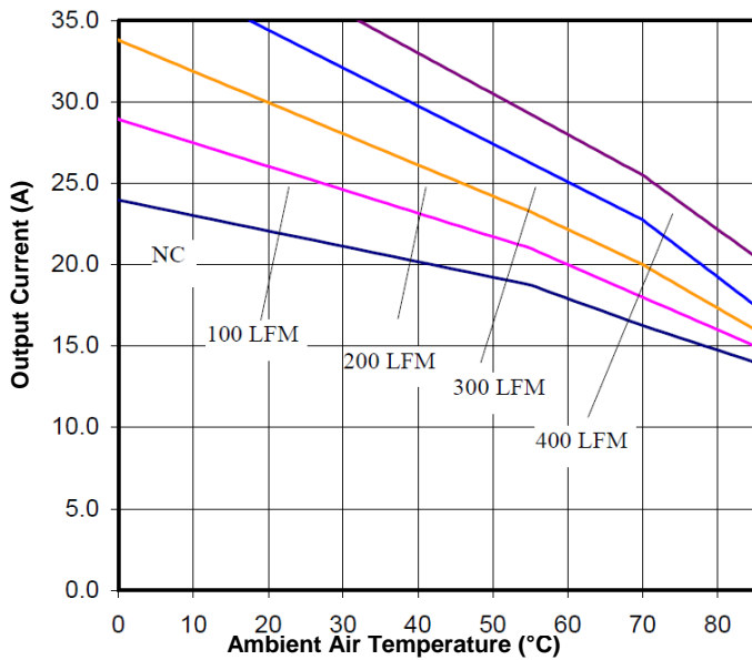
Figure 13. Current Derating Curve for Airflow Direction 4 (Ref. Fig. 14 for Airflow Direction; typical Vin, open frame unit using soldering interface)
