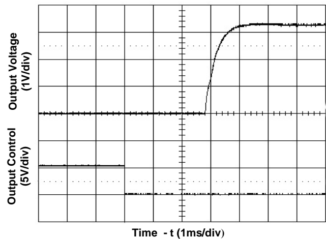
Figure 4. Start-Up from Enable Control Input voltage 48V, Output current 0A
