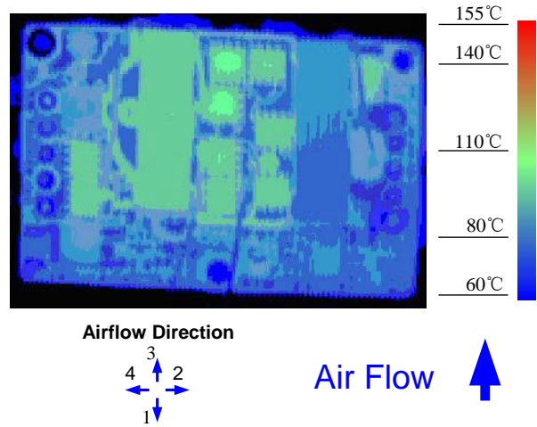
Figure 12. Thermal Image for Airflow Direction 3 (28A output, 55°C ambient, 200 LFM, typical Vin, open frame unit using soldering interface)
