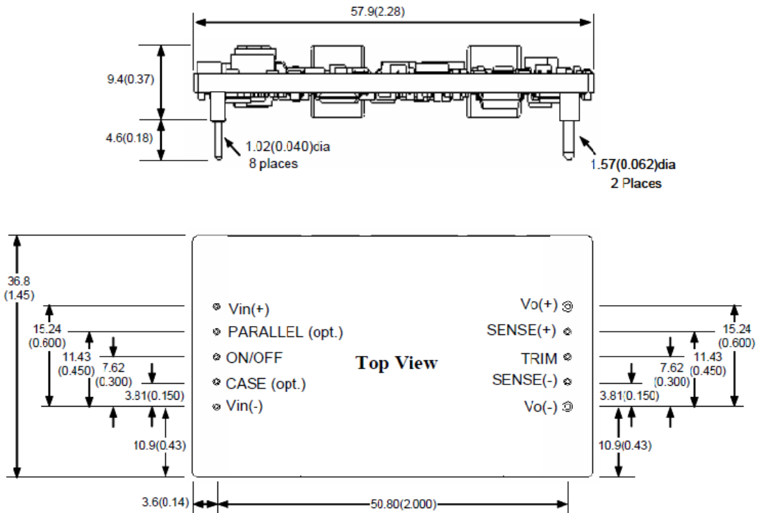
Figure 22. Open frame converter
