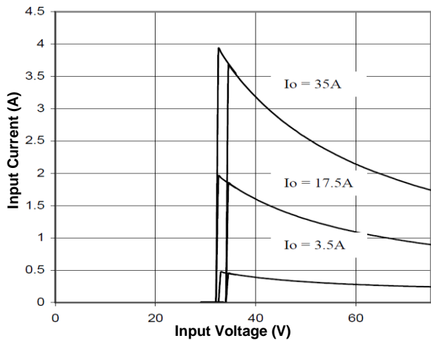
Figure 9. Input Characteristics
