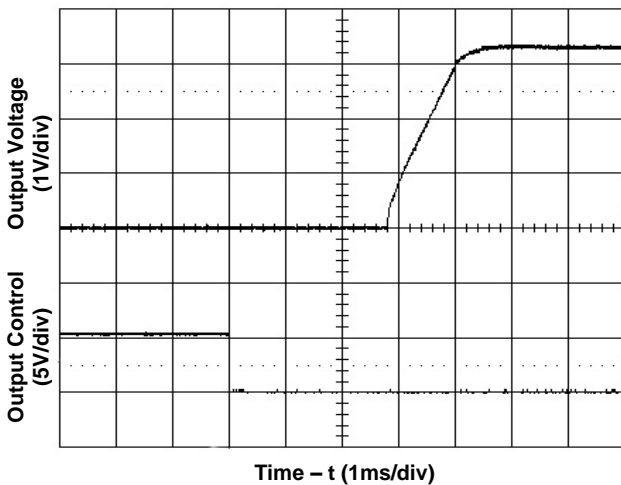
Figure 3. Start-Up from Enable Control Input voltage 48V, Output current 35A
