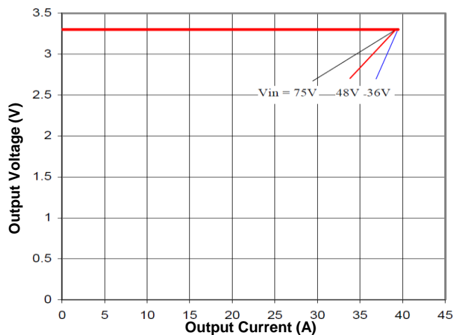
Figure 10. Output Characteristics
