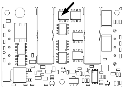
Figure 21. Temperature Monitoring Location
