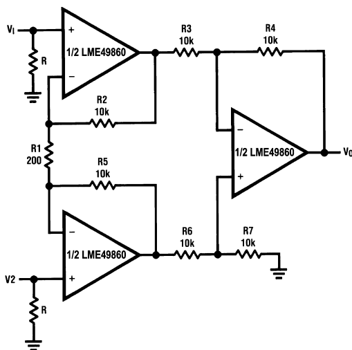
Figure 21. RIAA Preamp
