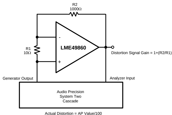
Figure 5. THD+N and IMD Distortion Test Circuit
