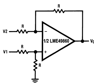
Figure 11. Balanced to Single Ended Converter
