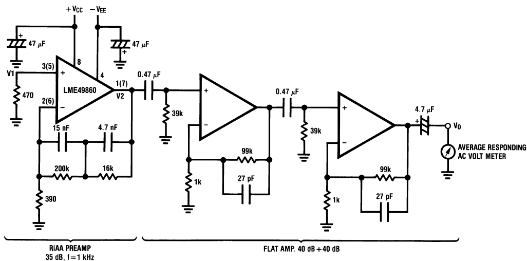
Figure 6. Noise Measurement Circuit Total Gain: 115 dB @f = 1 kHz Input Referred Noise Voltage: e_n = V_0/560,000 (V)
