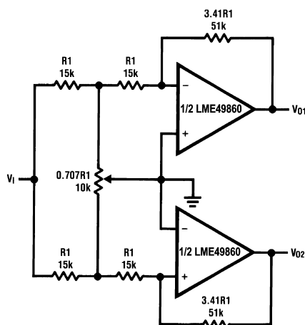
Figure 18. 2 Channel Panning Circuit (Pan Pot)
