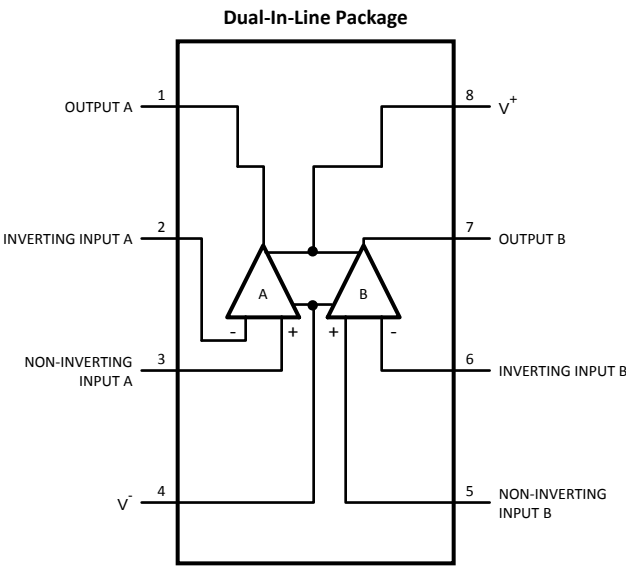
Figure 2. See NS Package Number — N08E
