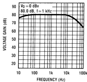
Figure 8. Flat Amp Voltage Gain vs Frequency
