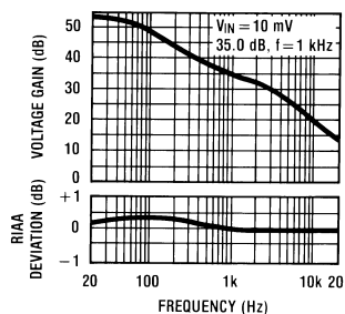
Figure 7. RIAA Preamp Voltage Gain, RIAA Deviation vs Frequency
