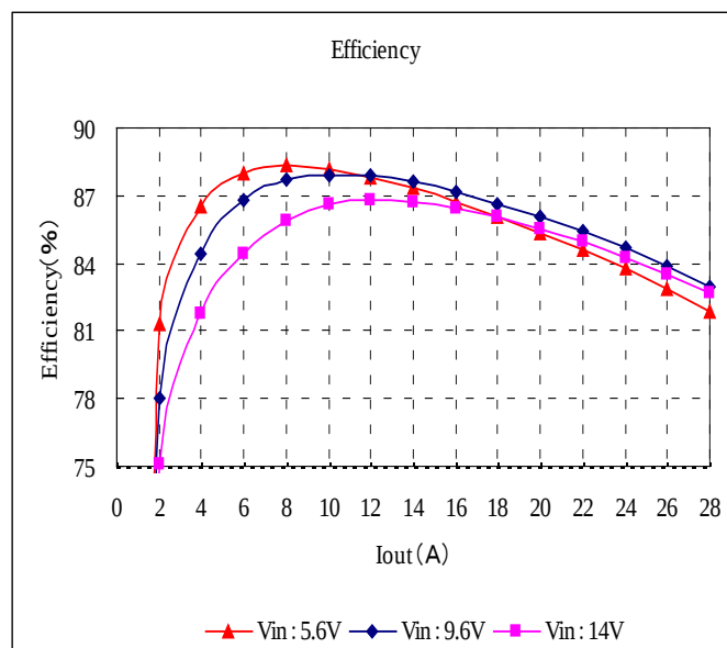
Fig. 12-3-14. Efficiency v.s. Output Current
