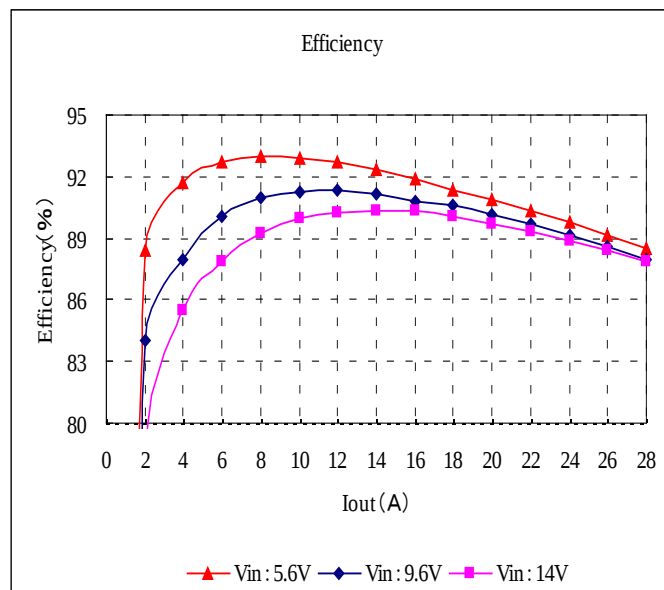
Fig. 12-3-5. Efficiency v.s. Output Current
