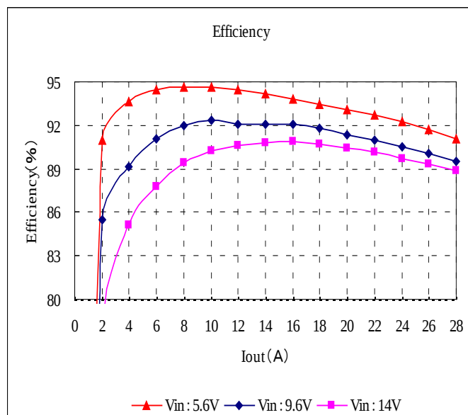
Fig. 12-3-2. Efficiency v.s. Output Current
