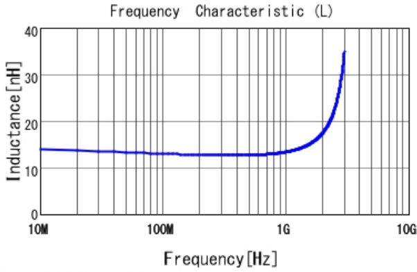
LQG15WH13NG02 L
