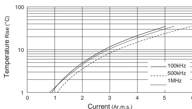
Ripple Current
