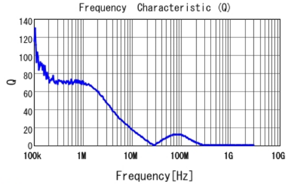
■ FDVE0640-H-3R3M Q
