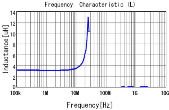
■ FDVE0640-H-3R3M L
