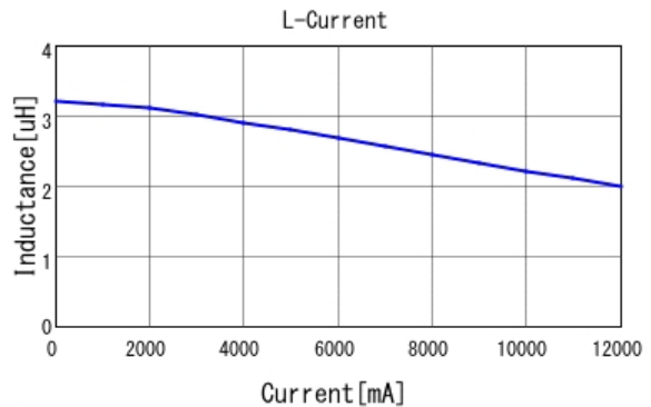
■ FDVE0640-H-3R3M L-Current 20degC
