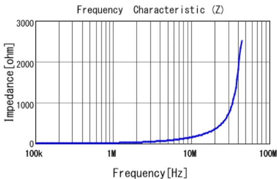
DFE201612PD-2R2M |Z|
