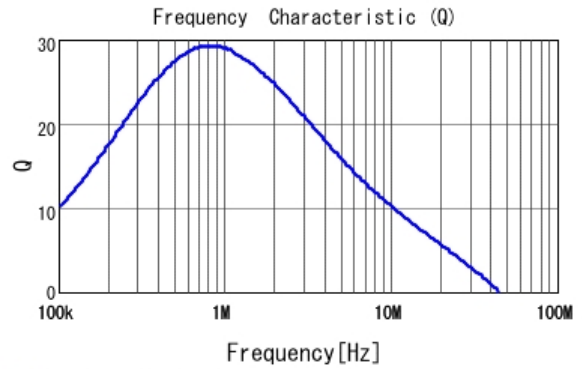
DFE201612PD-2R2M Q
