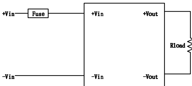
Figure 2. Input Fusing
