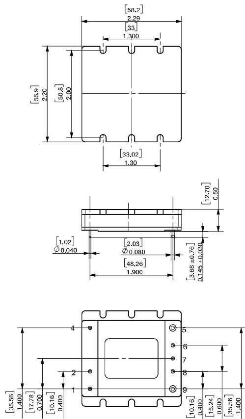
SLOTTED / FLANGED BASEPLATE
