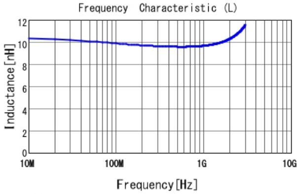
LQW04AN9N6D00 L
