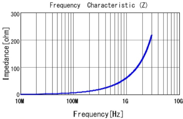
LQW04AN9N6D00 |Z|
