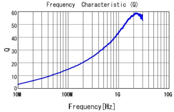
LQW04AN9N6D00 Q
