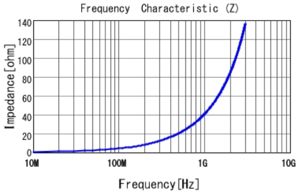
LQW04AN6N6D00 |Z|
