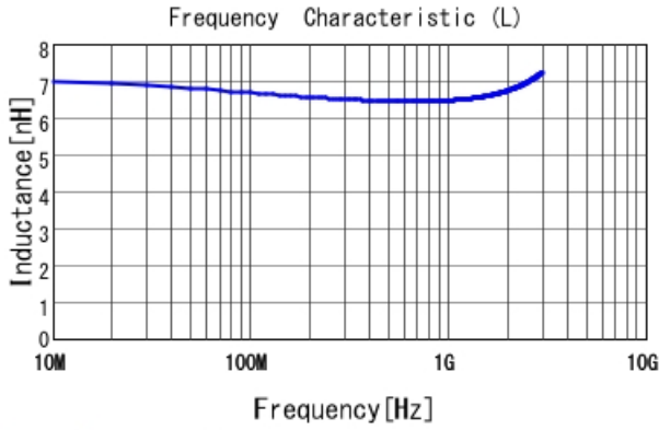
LQW04AN6N6D00 L
