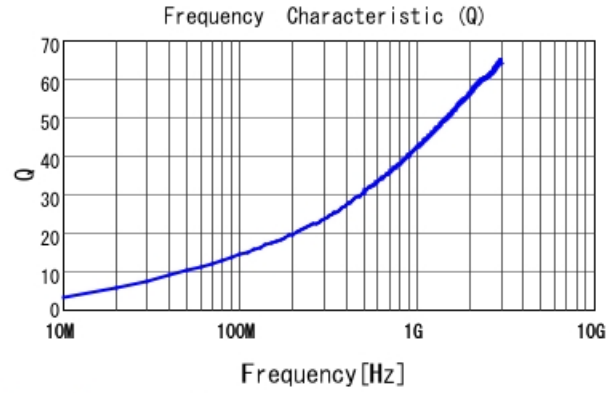
LQW04AN6N6D00 Q
