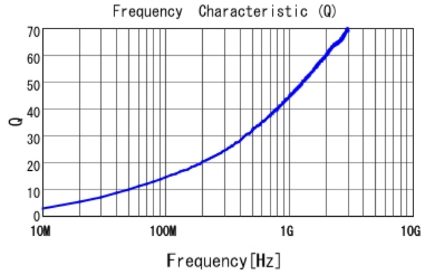
LQW04AN6N3D00 Q
