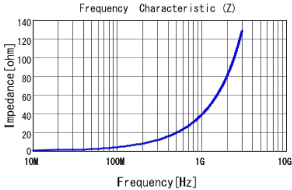
LQW04AN6N3D00 |Z|
