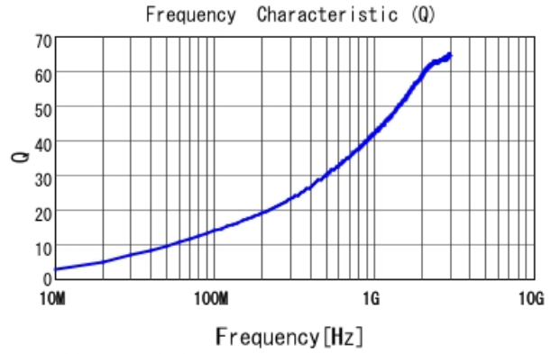
LQW04AN6N1C00 Q
