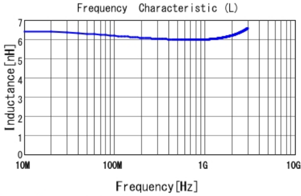
LQW04AN6N1C00 L
