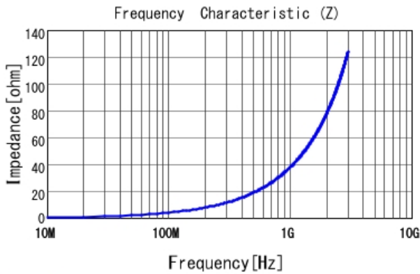
LQW04AN6N1C00 |Z|
