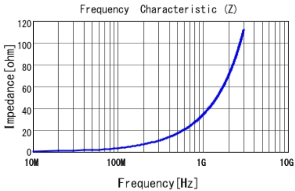
LQW04AN5N5C00 |Z|
