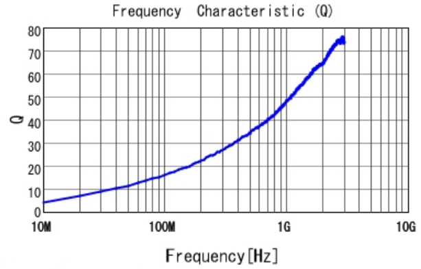
LQW04AN5N5C00 Q
