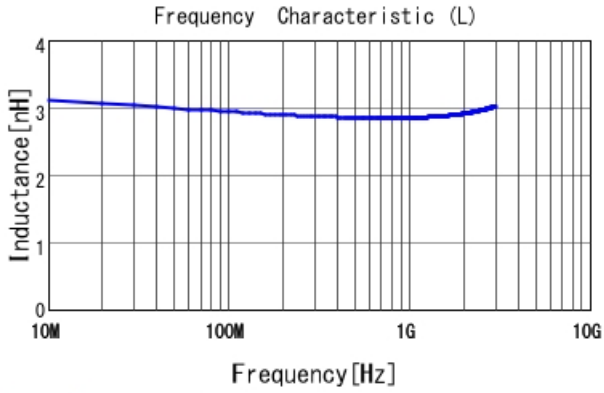
LQW04AN2N8D00 L
