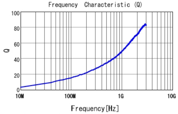
LQW04AN2N8D00 Q
