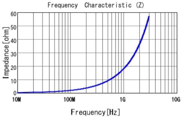
LQW04AN2N8D00 |Z|
