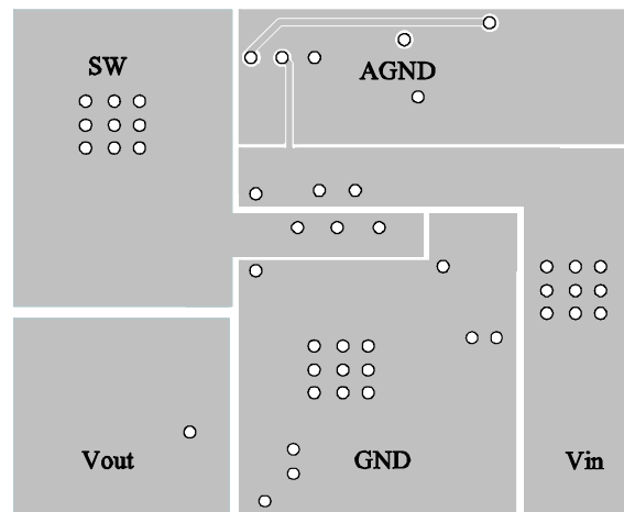
Bottom Layer Figure : PCB Layout
