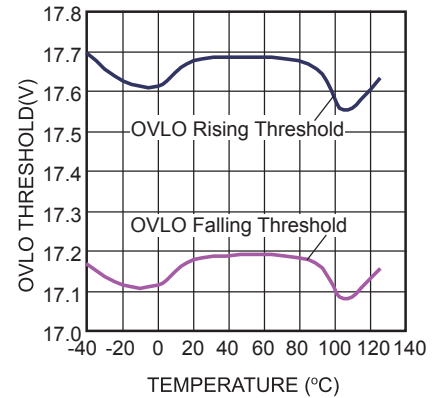
OVLO Threshold vs. Temperature
