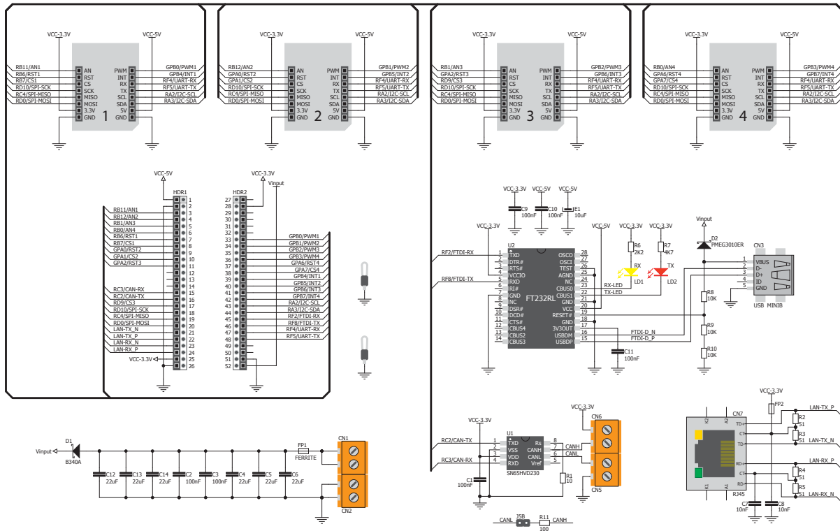
Figure 1-2: mikromedia+ SHIELD for PIC32MX7® schematic
