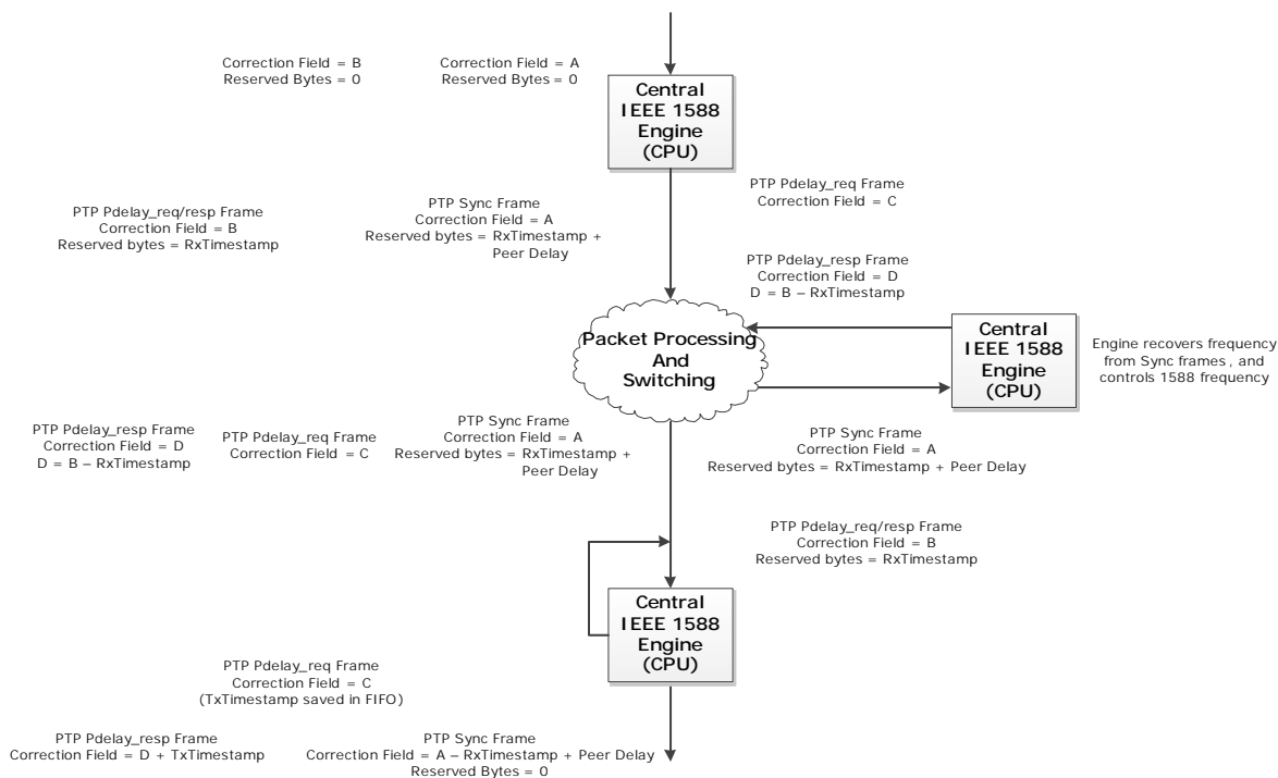
Figure 26 • One-Step Peer-to-Peer Transparent Clock Mode B
