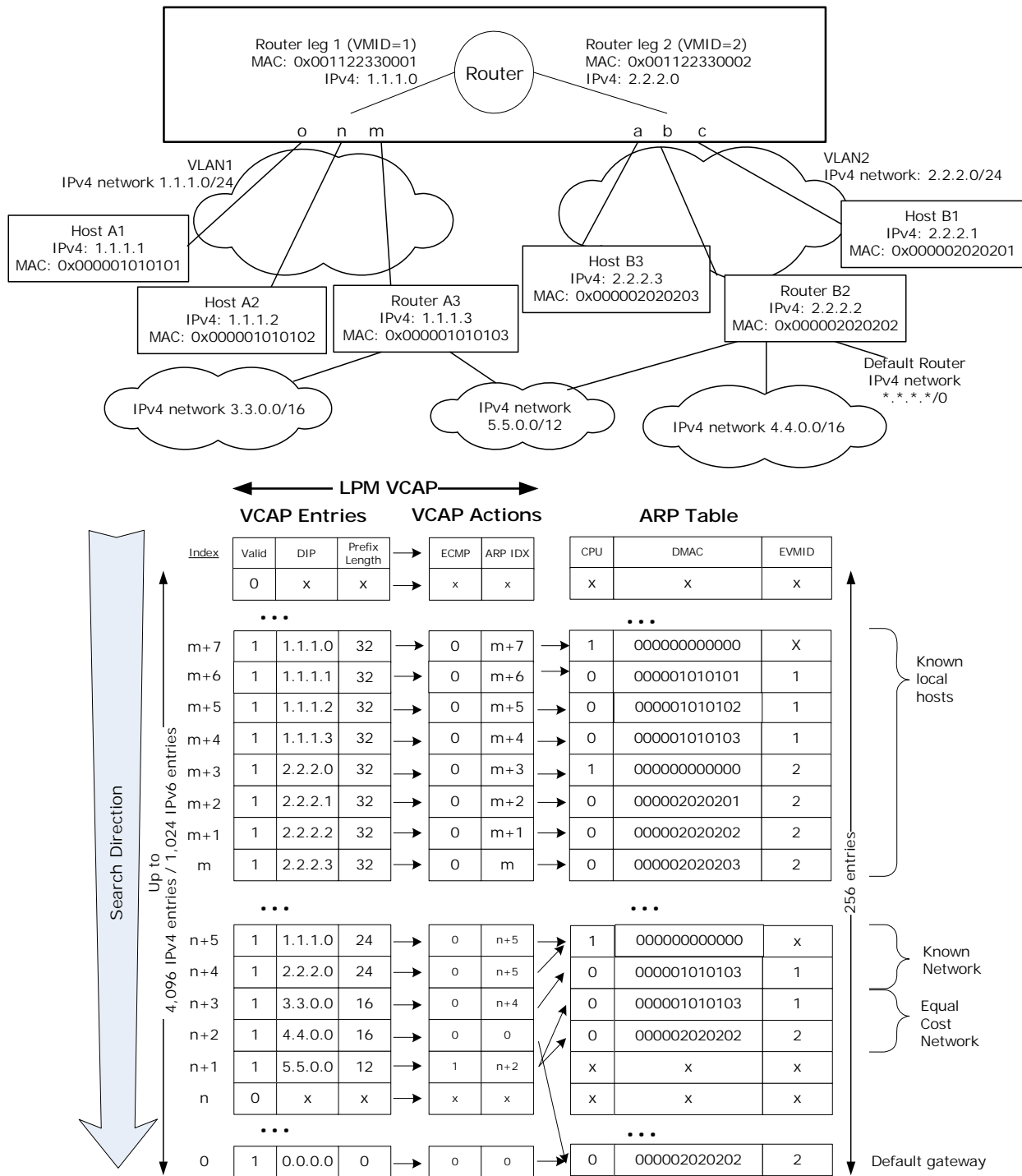
Figure 35 • IP Unicast Routing Example
