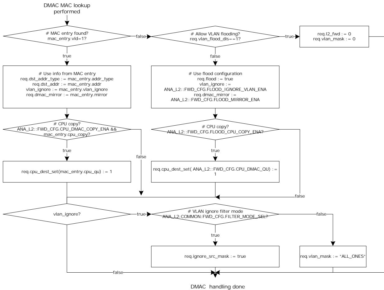
Figure 39 • DMAC Lookup
