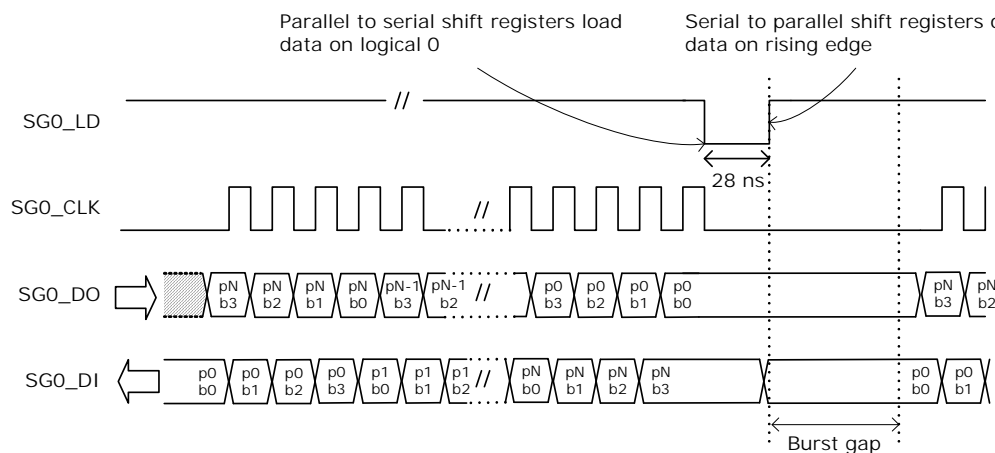
Figure 127 • SIO Timing
