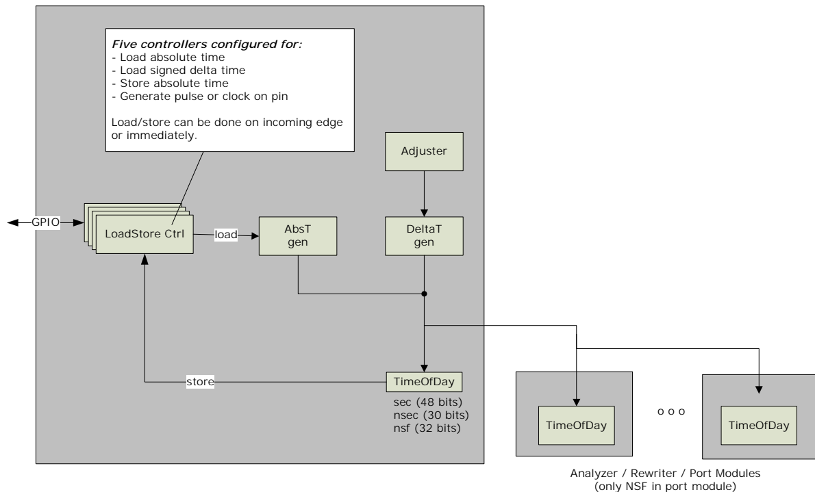
Figure 87 • Timing Distribution
