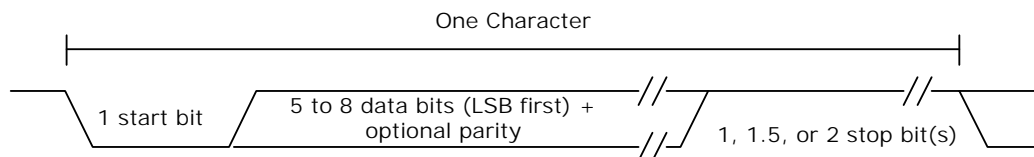
Figure 124 • UART Timing
