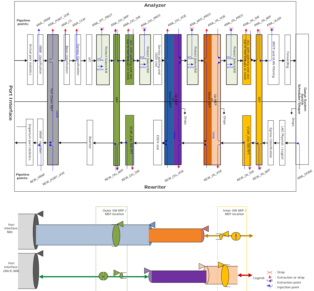
Figure 22 • Processing Flow
