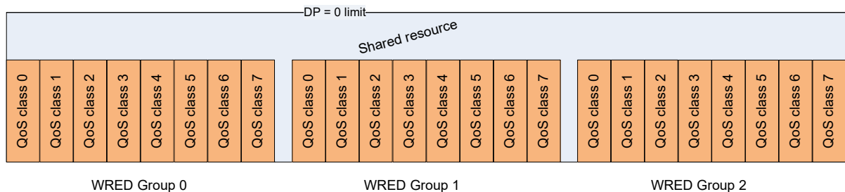
Figure 60 • WRED Sharing
