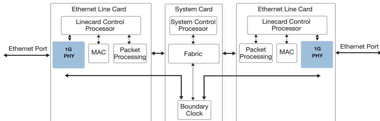
Figure 56 • TC and BC Linecard Application
