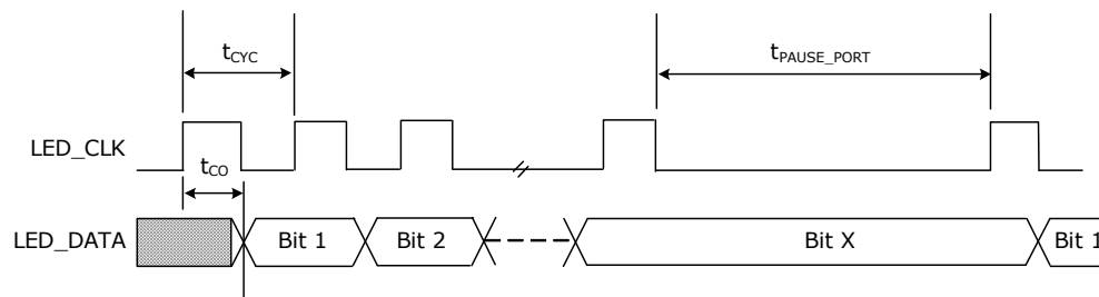
Figure 120 • Basic Serial LED Timing
