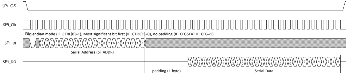
Figure 102 • SPI Read Cycle
