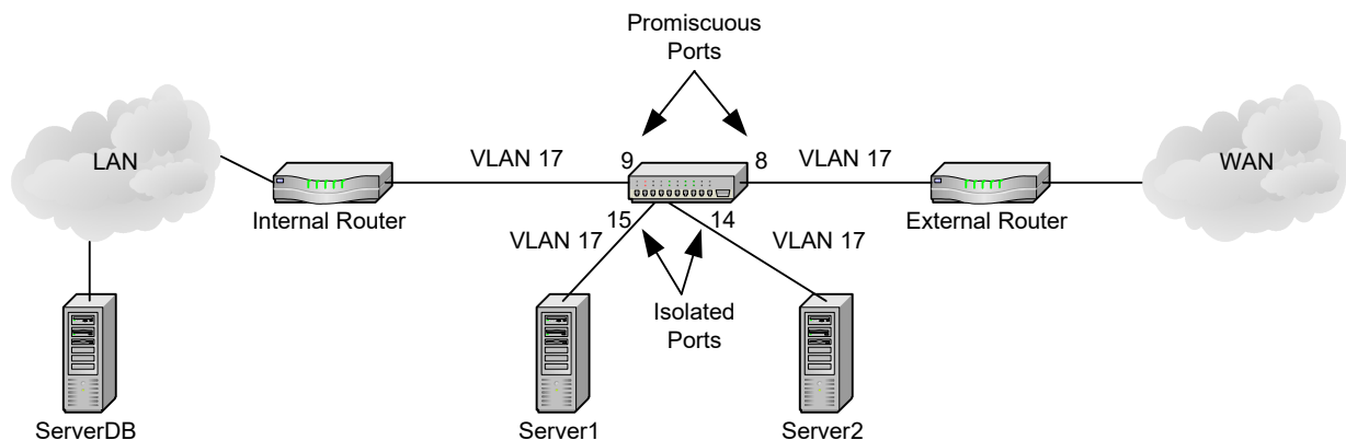
Figure 72 • DMZ Example for Private VLAN
