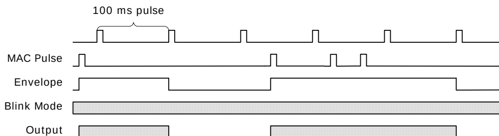
Figure 67 • Link Activity Timing
