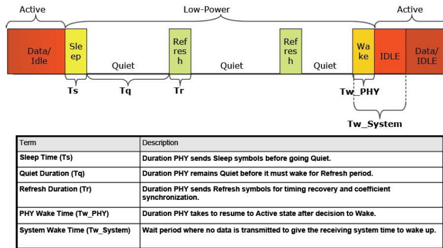
Figure 10 • Energy Efficient Ethernet
