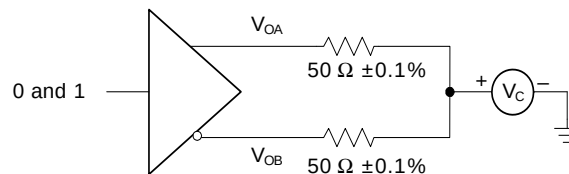
Figure 82 • SGMII DC Driver Output Impedance Test Circuit
