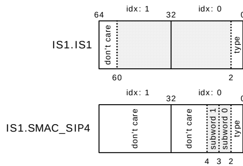
Figure 26 • Action Layout in Register Example
