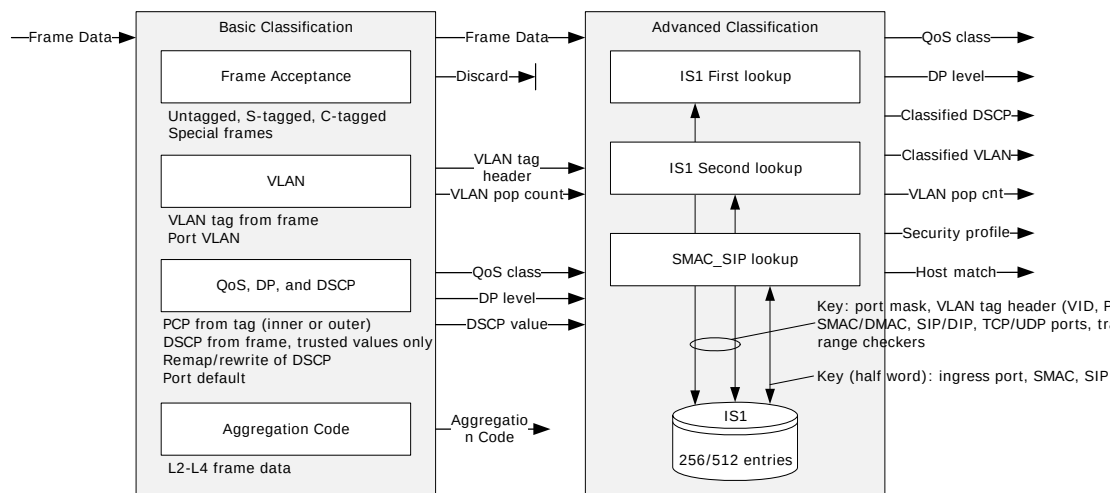
Figure 2 • Basic and Advanced Frame Classification
