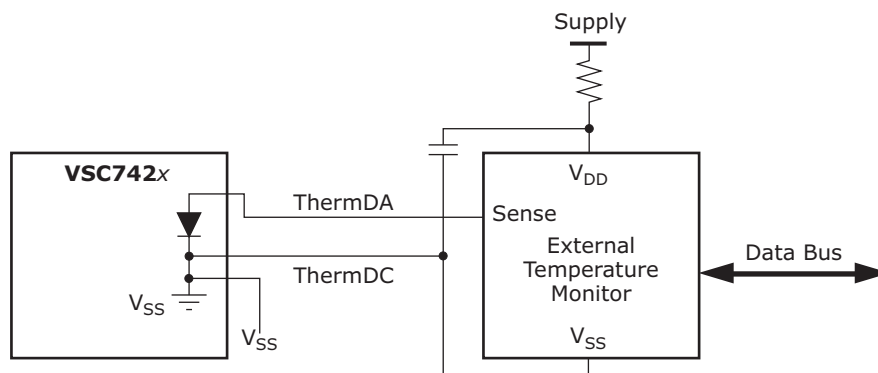
Figure 116 • External Temperature Monitor Connection
