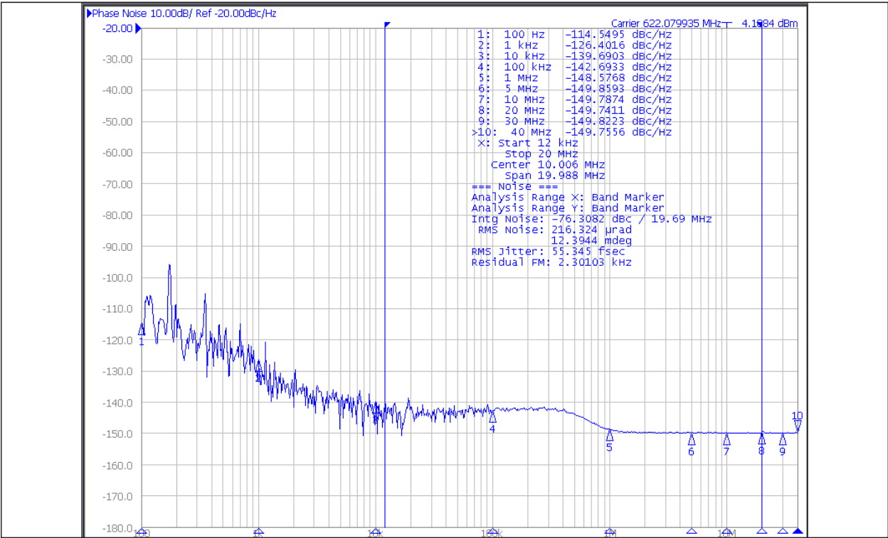
FIGURE 3-5: 622 MHz Phase Jitter, Device.
