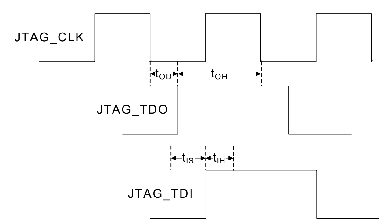
FIGURE 34-15: JTAG SETUP &amp; HOLD PARAMETERS
