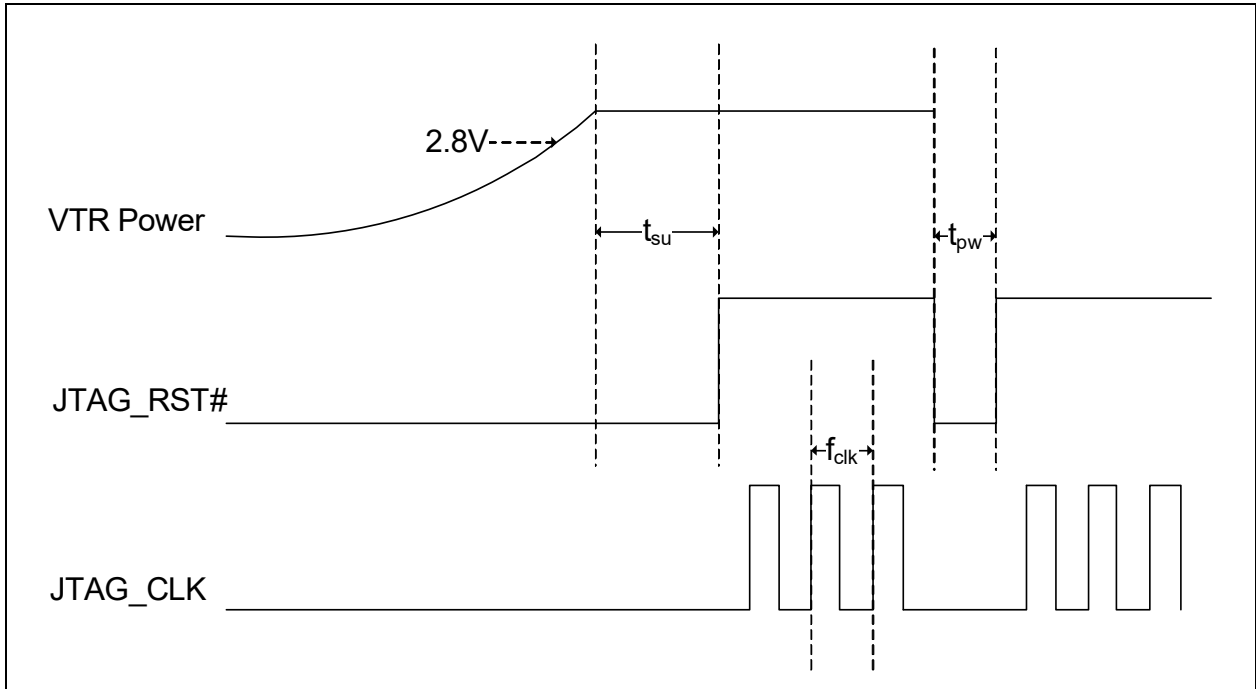
FIGURE 34-14: JTAG POWER-UP &amp; ASYNCHRONOUS RESET TIMING
