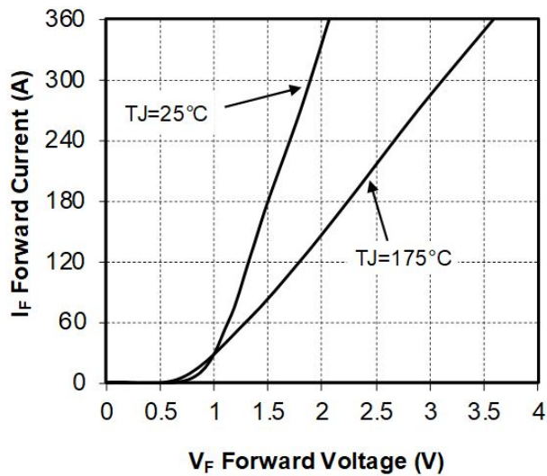
Figure 1-16. Forward Characteristics
