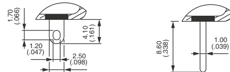
Solder lugs
