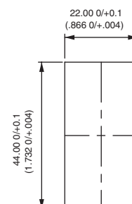
PANEL CUT-OUT
