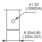
Normalized quick-connect
