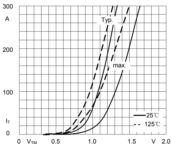
Fig5. Forward Characteristics
