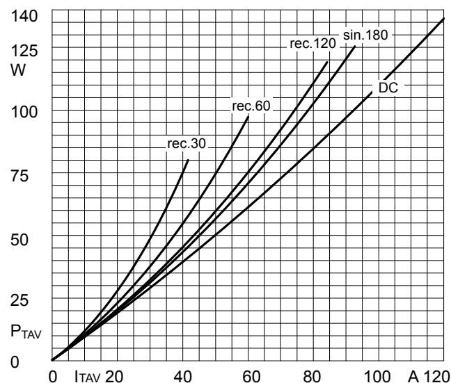
Fig1. Power dissipation
