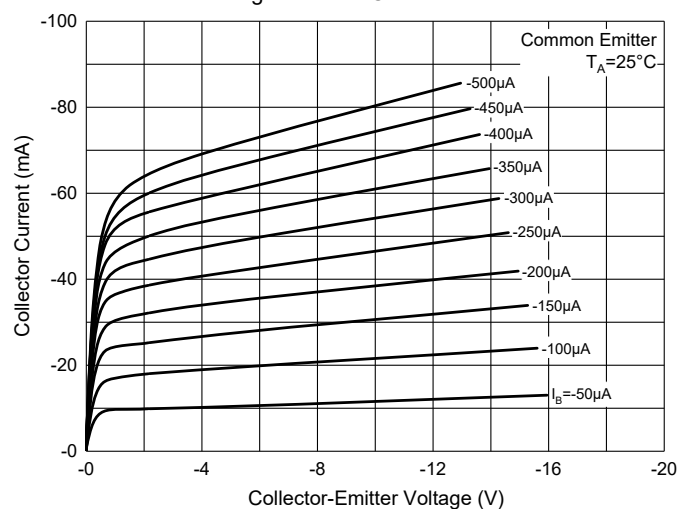
Fig. 7 - Static Characteristics
