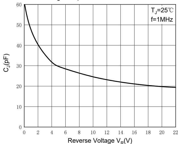
Fig.6: Capacitance Characteristics
