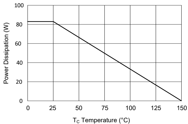
Fig.11 - PD Dissipation
