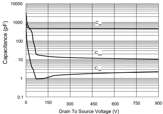
Fig.5 - Capacitance Characteristics
