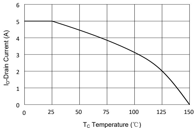
Fig.10 - Drain Current
