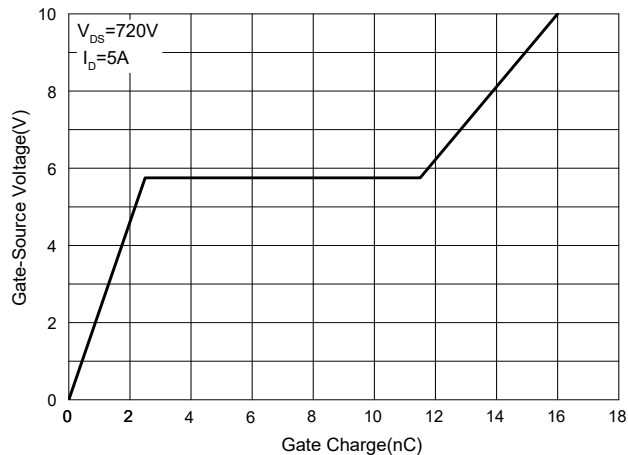
Fig. 6 - Gate Charge
