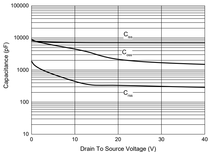
Fig. 5 - Capacitance Characteristics
