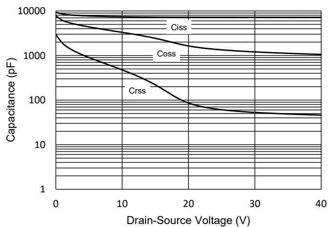
Fig.5 Capacitance Characteristics
