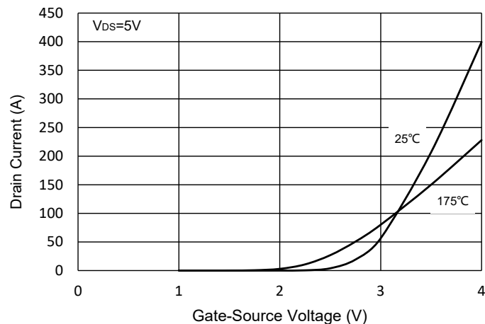
Fig.2 Transfer Characteristic
