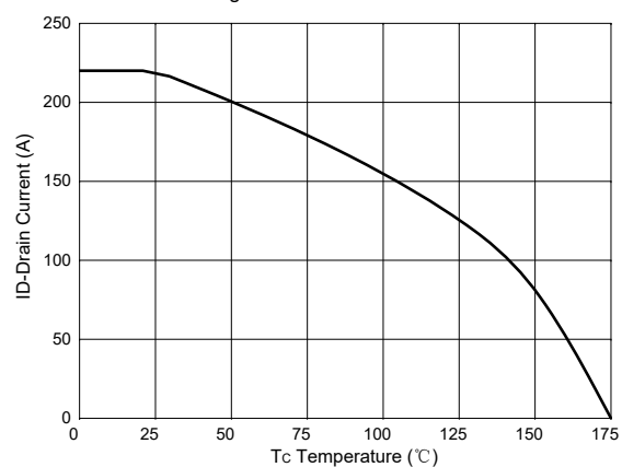
Fig. 10 - Drain Current
